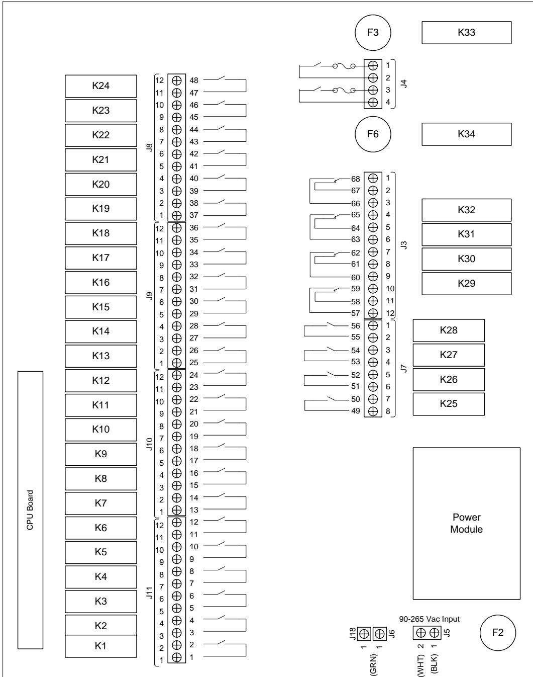
Figure 19: CT24-32 Relays and Terminals
