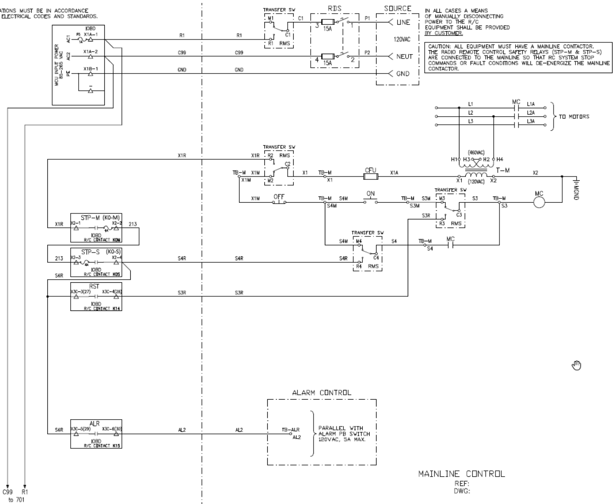
Figure 21 Example Typical non-PLd Mainline and Manual Remote Transfer Drawing
